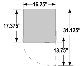
EXTERIOR DIMENSIONS
