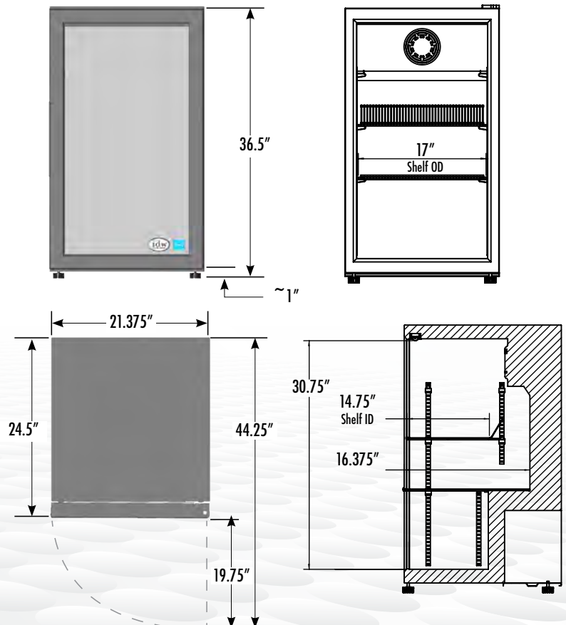
EXTERIOR DIMENSIONS
