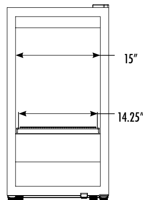
INTERIOR DIMENSIONS
