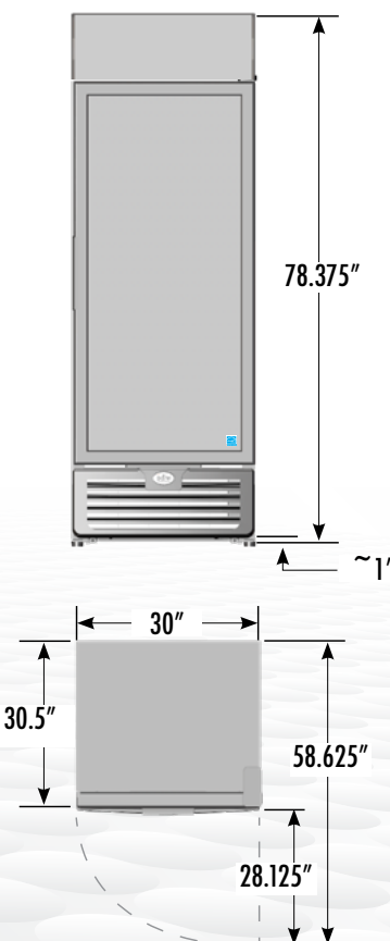
EXTERIOR DIMENSIONS
