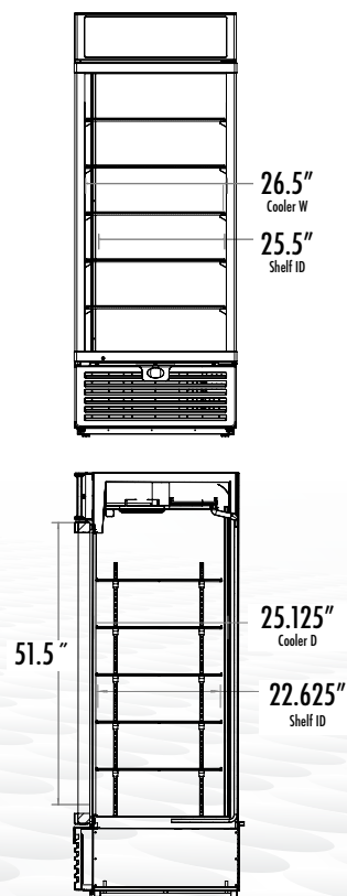
INTERIOR DIMENSIONS
