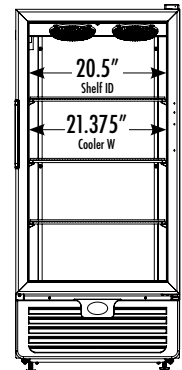
INTERIOR DIMENSIONS
