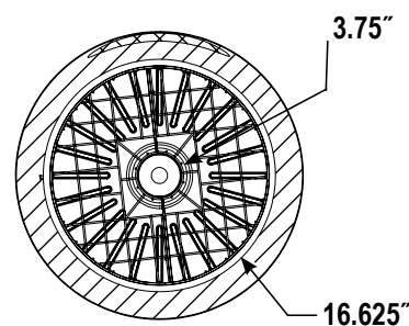
INTERIOR DIMENSIONS
