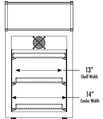
INTERIOR DIMENSIONS
