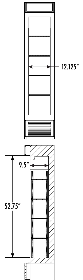
INTERIOR DIMENSIONS
