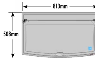
EXTERIOR DIMENSIONS
