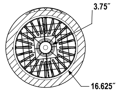
INTERIOR DIMENSIONS
