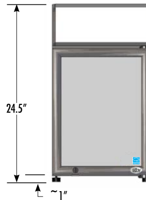
EXTERIOR DIMENSIONS
