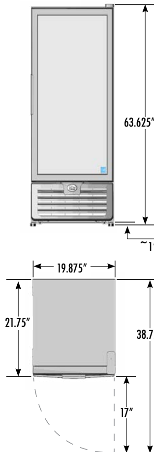
EXTERIOR DIMENSIONS
