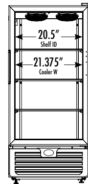
INTERIOR DIMENSIONS
