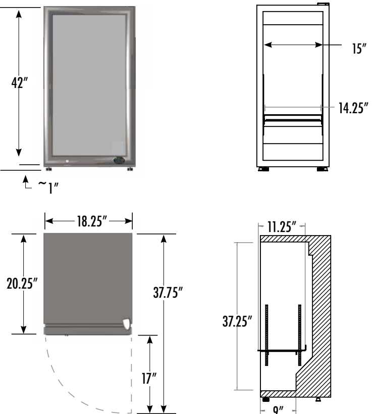
EXTERIOR DIMENSIONS
