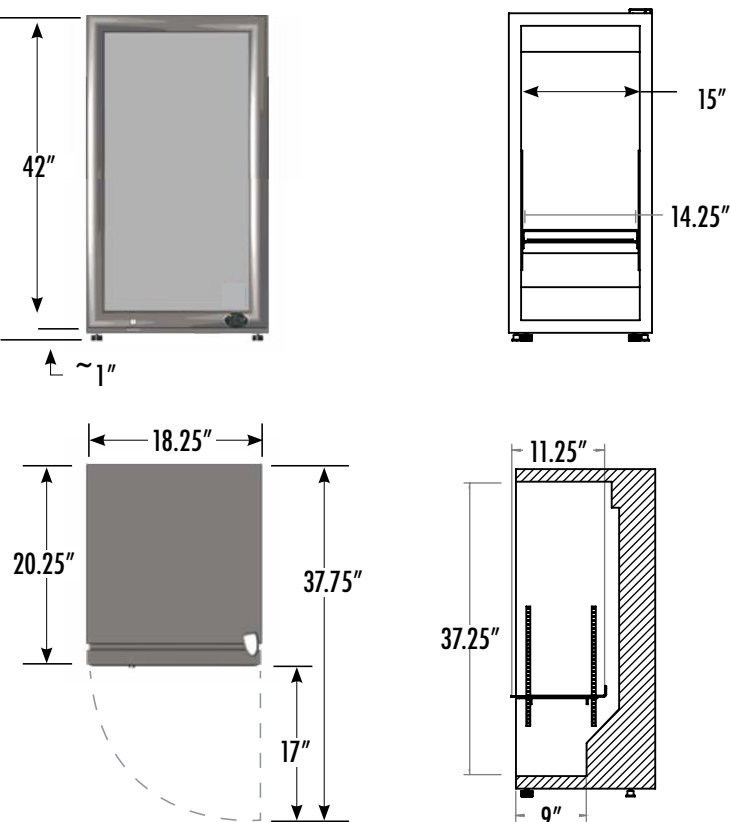
EXTERIOR DIMENSIONS
