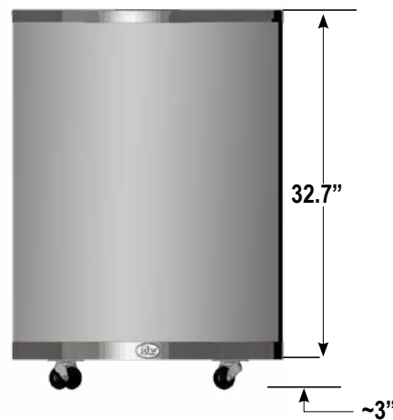
EXTERIOR DIMENSIONS
