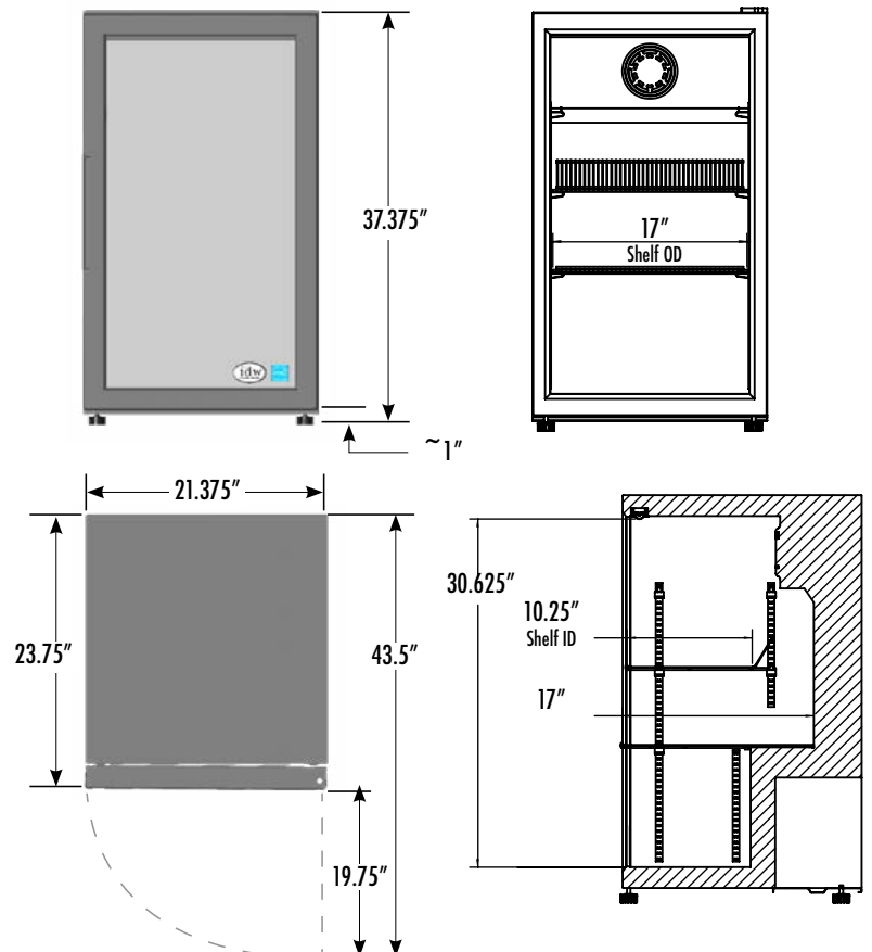
EXTERIOR DIMENSIONS
