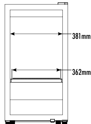
INTERIOR DIMENSIONS
