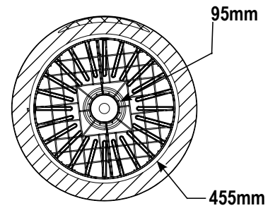
INTERIOR DIMENSIONS
