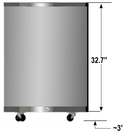
EXTERIOR DIMENSIONS
