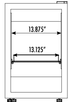
INTERIOR DIMENSIONS
