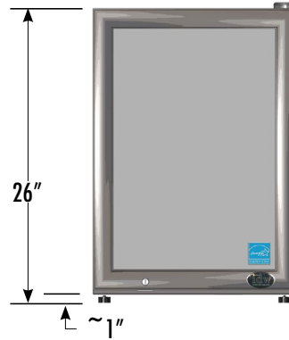
EXTERNAL DIMENSIONS
