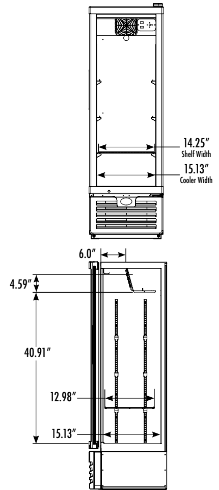
Internal Dimensions
