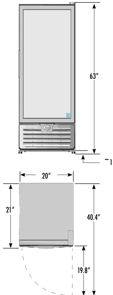
External Dimensions
