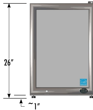
EXTERNAL DIMENSIONS
