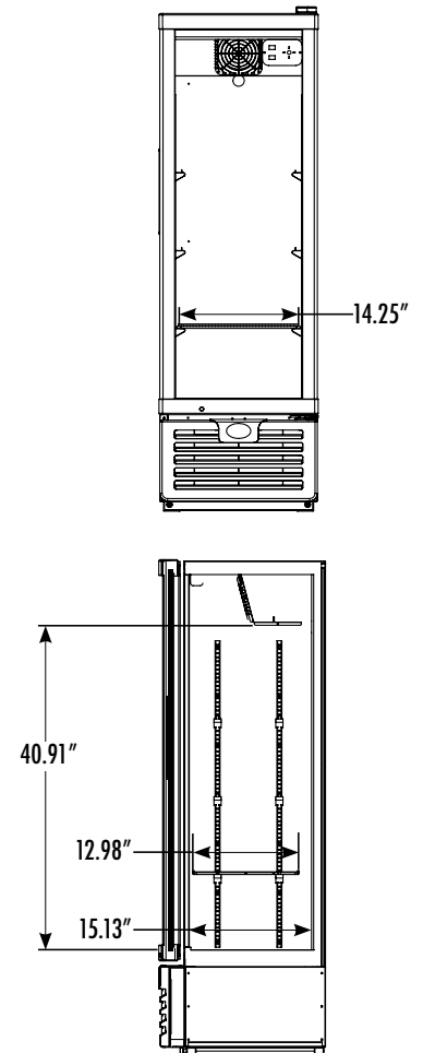
Internal Dimensions
