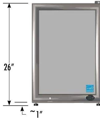
EXTERIOR DIMENSIONS
