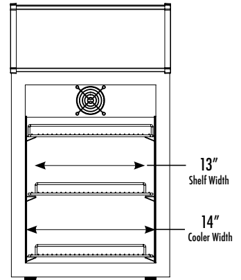
INTERIOR DIMENSIONS
