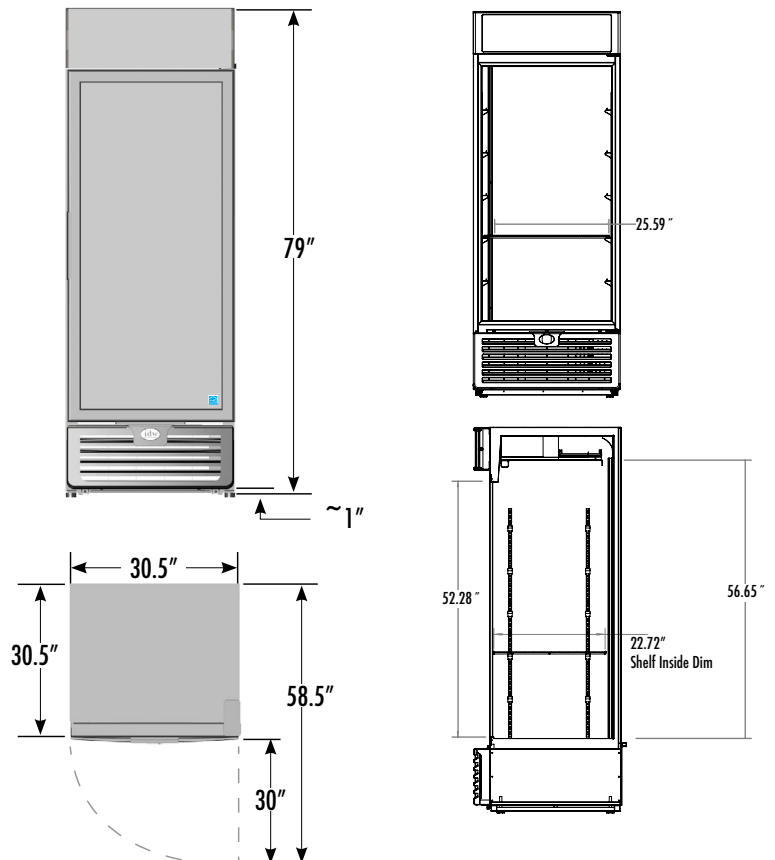
External Dimensions
