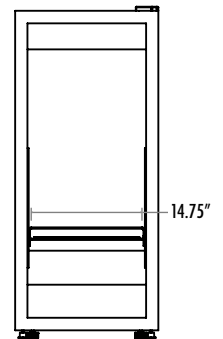
Internal Dimensions
